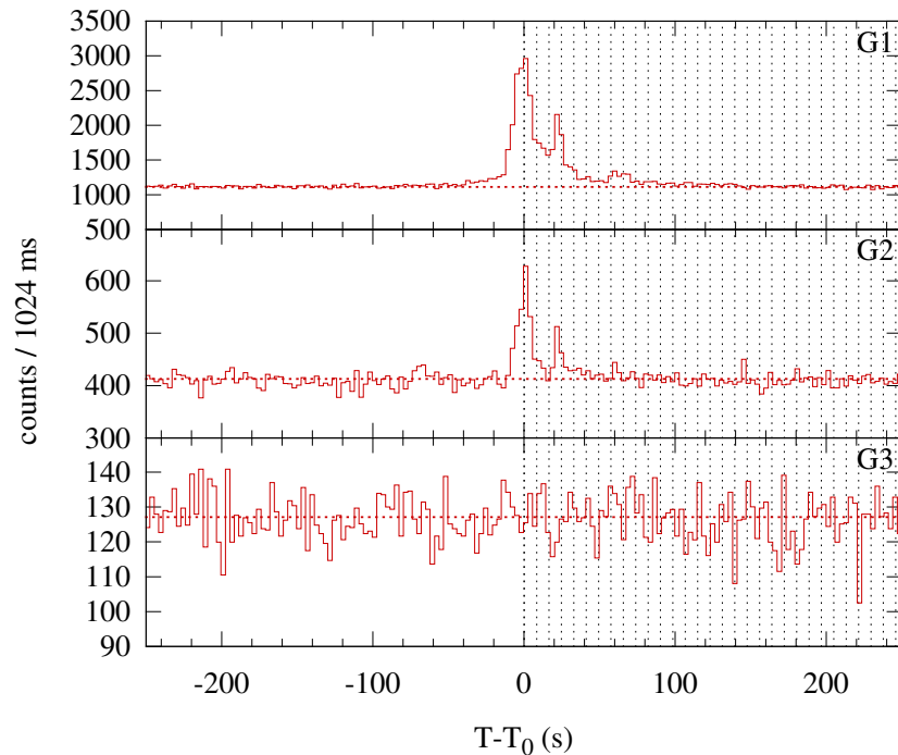
Konus-WIND S2 SOL2001-09-13T16:00 (C7.0) T 0 = 57639.287 s UT (16:00:39.287)
