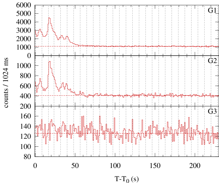
Konus-WIND S2 SOL2001-09-13T19:50 (C5.8) T 0 = 71415.910 s UT (19:50:15.910)
