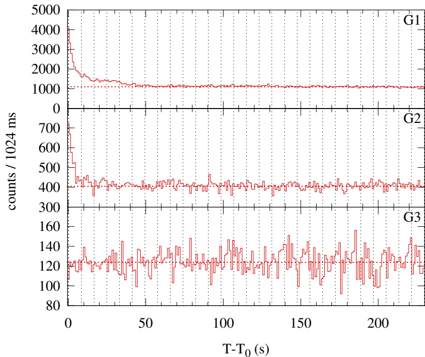
Konus-WIND S2 SOL2001-09-16T07:43 (C4.5) T 0 = 27828.114 s UT (07:43:48.114)
