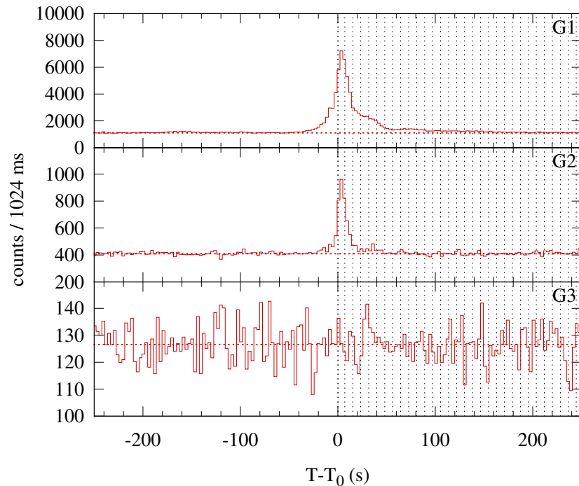
Konus-WIND S2 SOL2001-09-18T00:06 (M1.4) T 0 = 375.629 s UT (00:06:15.629)
