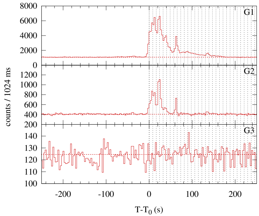
Konus-WIND S2 SOL2001-09-18T17:05 (M1.4) T_0 = 61522.203 s UT (17:05:22.203)
