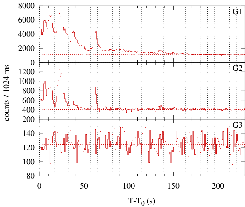
Konus-WIND S2 SOL2001-09-18T17:05 (M1.4) T_0 = 61522.203 s UT (17:05:22.203)
