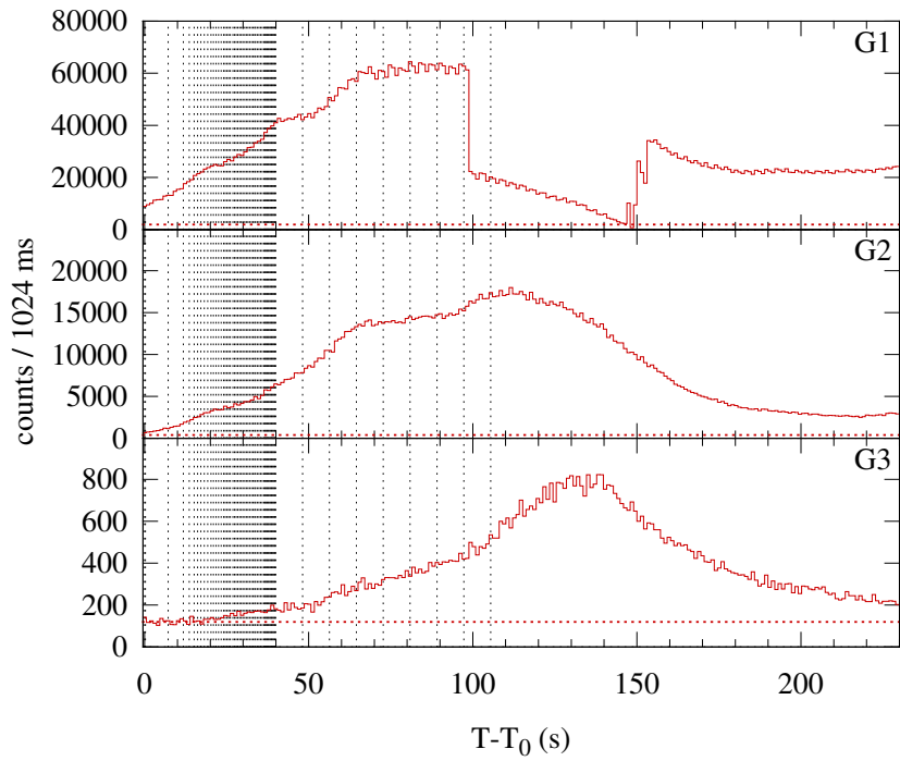
Konus-WIND S2 SOL2001-09-24T10:17 (X2.6) T_0 = 37073.525 s UT (10:17:53.525)
