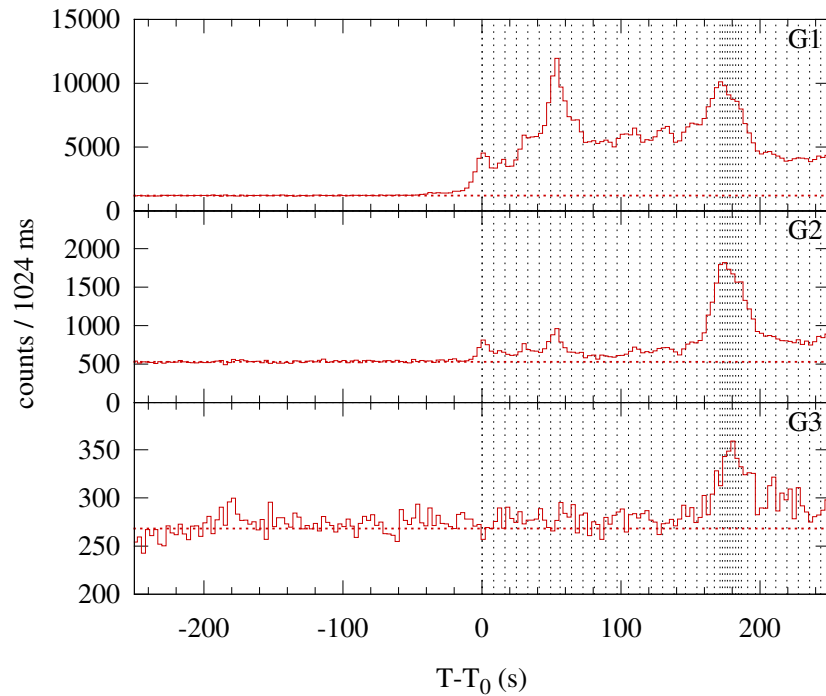
Konus-WIND S2 SOL2001-10-19T09:38 (M5.7) T_0 = 34719.982 s UT (09:38:39.982)
