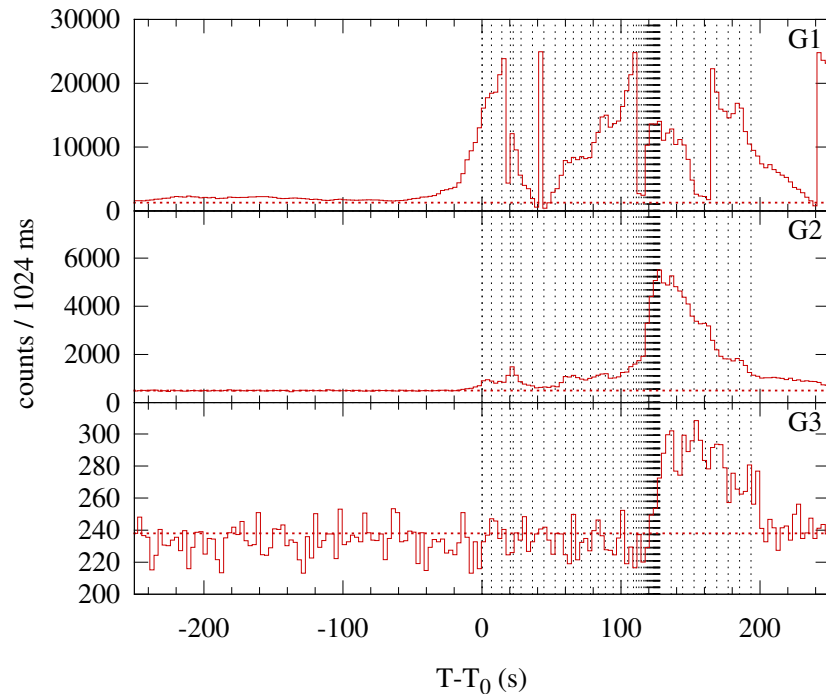
Konus-WIND S2 SOL2001-10-19T16:22 (X1.6) T_0 = 58963.618 s UT (16:22:43.618)
