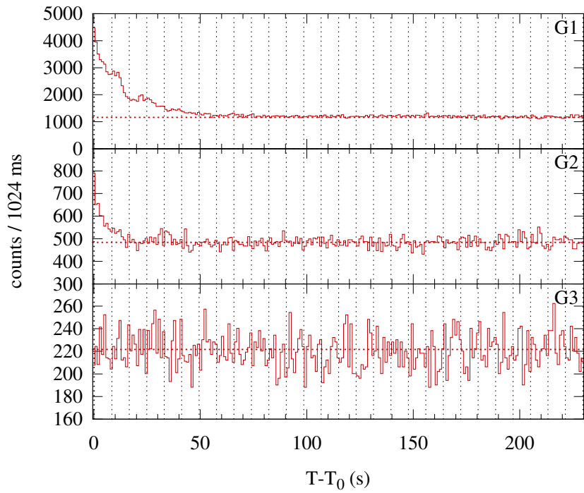
Konus-WIND S2 SOL2001-10-25T05:18 (C5.2) T_0 = 19106.823 s UT (05:18:26.823)
