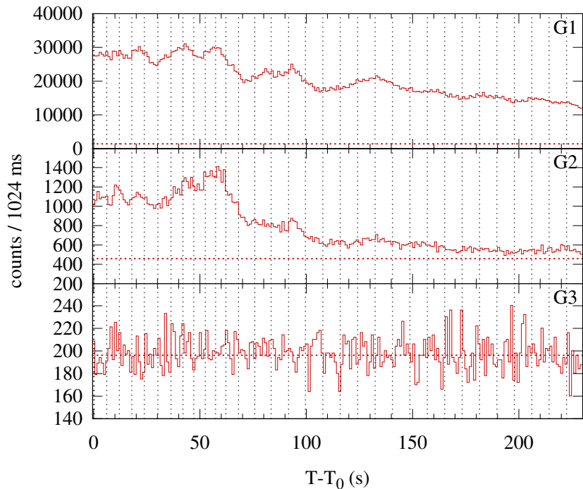
Konus-WIND S2 SOL2001-10-25T14:51 (X1.3) T_0 = 53490.205 s UT (14:51:30.205)
