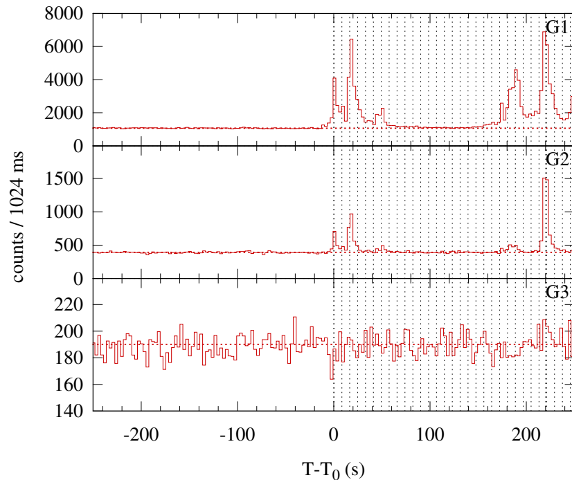
Konus-WIND S1 SOL2001-10-26T14:30 (M2.0) T 0 = 52221.707 s UT (14:30:21.707)
