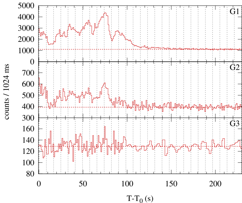
Konus-WIND S2 SOL2001-10-30T12:18 (C7.4) T_0 = 44310.975 s UT (12:18:30.975)
