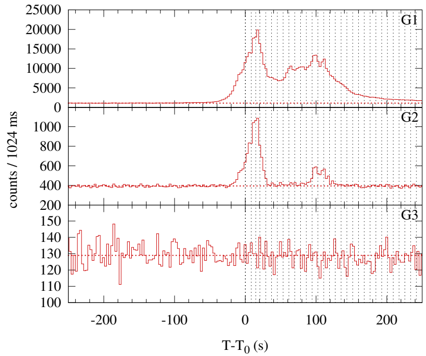
Konus-WIND S2 SOL2001-10-31T08:03 (M3.2) T 0 = 29017.7 s UT (08:03:37.7)
