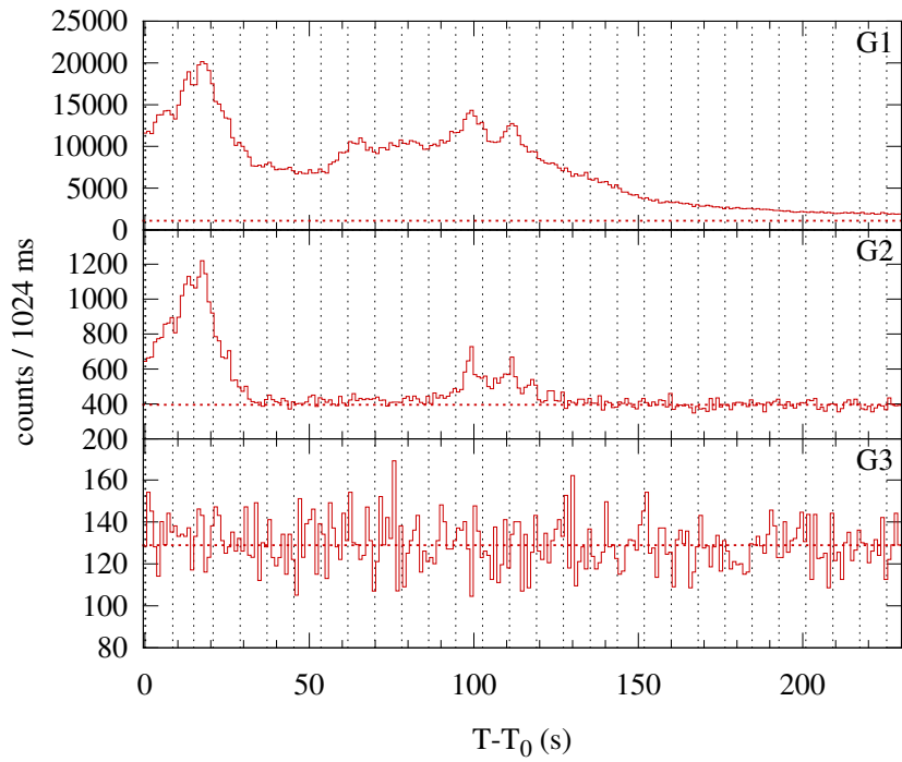
Konus-WIND S2 SOL2001-10-31T08:03 (M3.2) T 0 = 29017.7 s UT (08:03:37.7)
