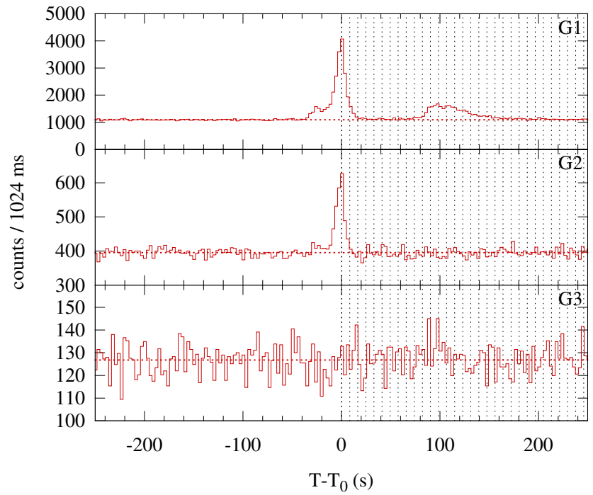
Konus-WIND S2 SOL2001-11-04T06:41 (C8.4) T 0 = 24072.935 s UT (06:41:12.935)
