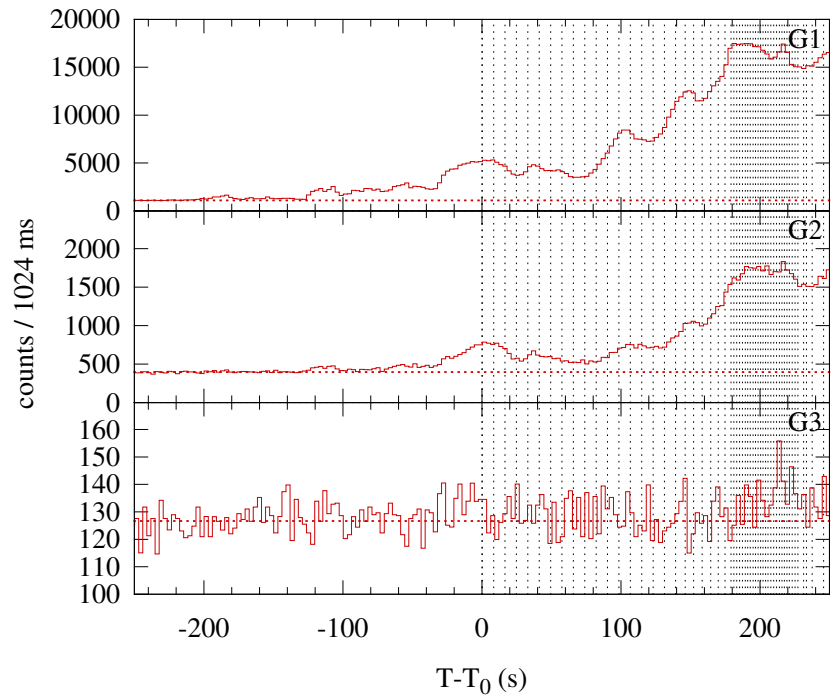
Konus-WIND S2 SOL2001-11-04T16:06 (X1.0) T_0 = 57968.876 s UT (16:06:08.876)
