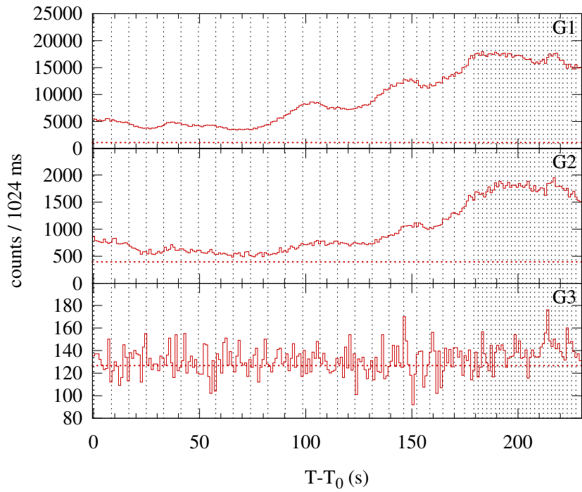
Konus-WIND S2 SOL2001-11-04T16:06 (X1.0) T_0 = 57968.876 s UT (16:06:08.876)
