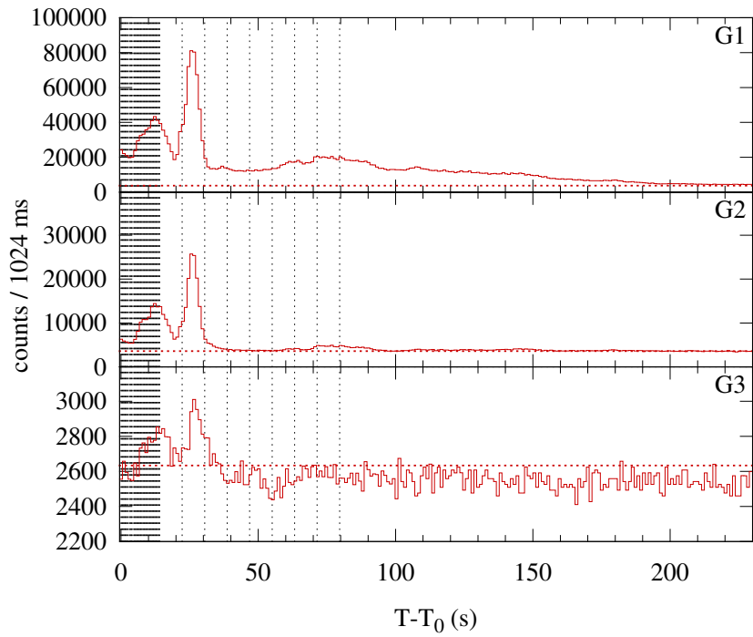
Konus-WIND S2 SOL2001-11-08T07:02 (M9.1) T_0 = 25345.203 s UT (07:02:25.203)
