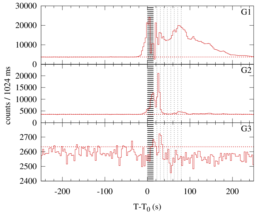
Konus-WIND S2 SOL2001-11-08T07:02 (M9.1) T_0 = 25345.203 s UT (07:02:25.203)
