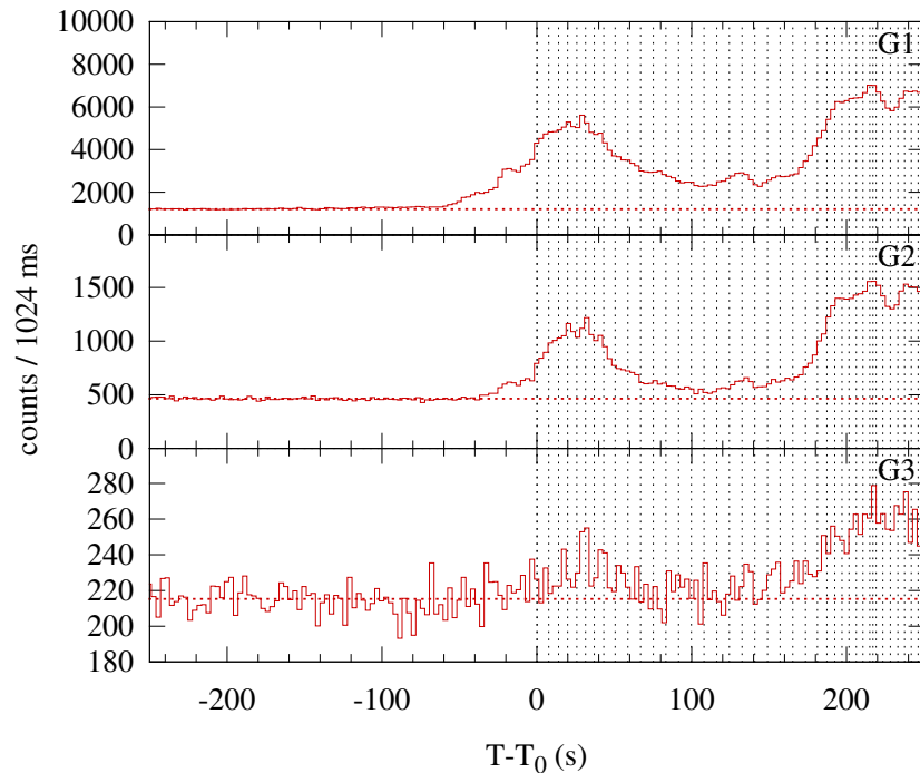
Konus-WIND S2 SOL2001-11-22T20:23 (M3.8) T_0 = 73390.698 s UT (20:23:10.698)
