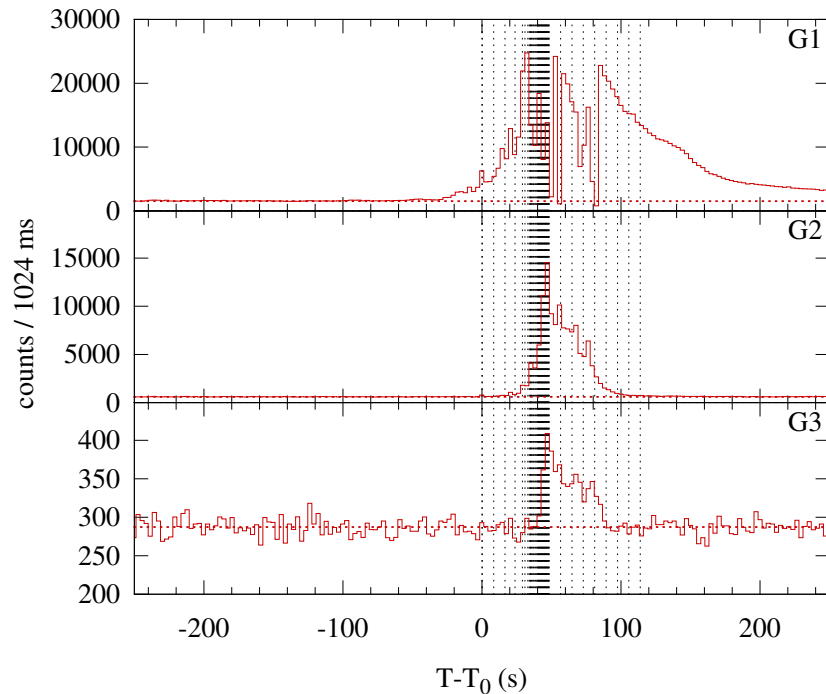
Konus-WIND S2 SOL2001-11-28T16:33 (M6.9) T 0 = 59586.719 s UT (16:33:06.719)
