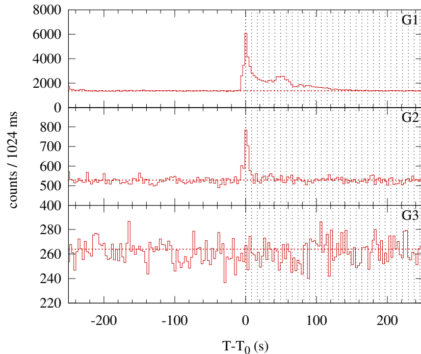
Konus-WIND S2 SOL2001-11-29T05:21 (C8.8) T_0 = 19271.612 s UT (05:21:11.612)
