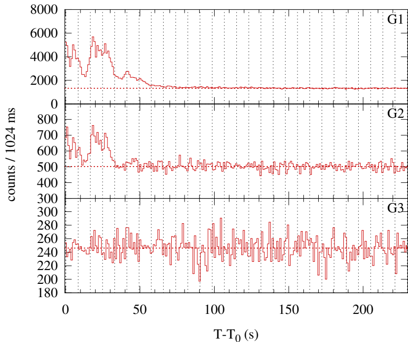
Konus-WIND S2 SOL2001-11-29T14:03 (C7.6) T_0 = 50600.999 s UT (14:03:20.999)
