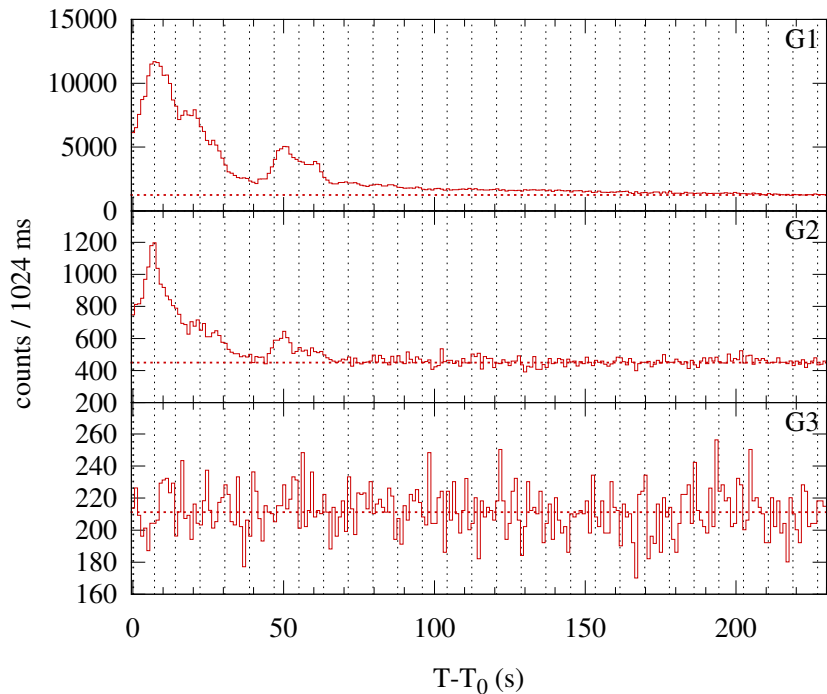
Konus-WIND S2 SOL2001-12-01T06:49 (M2.2) T_0 = 24542.533 s UT (06:49:02.533)
