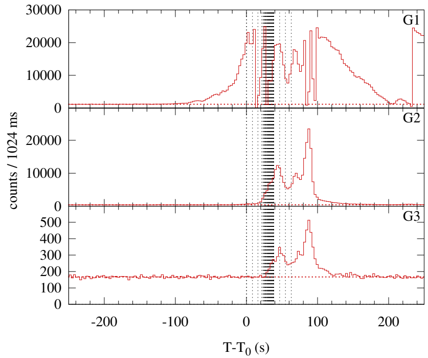
Konus-WIND S2 SOL2001-12-11T08:03 (X2.8) T_0 = 29018.854 s UT (08:03:38.854)
