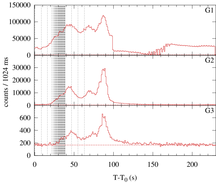
Konus-WIND S2 SOL2001-12-11T08:03 (X2.8) T_0 = 29018.854 s UT (08:03:38.854)
