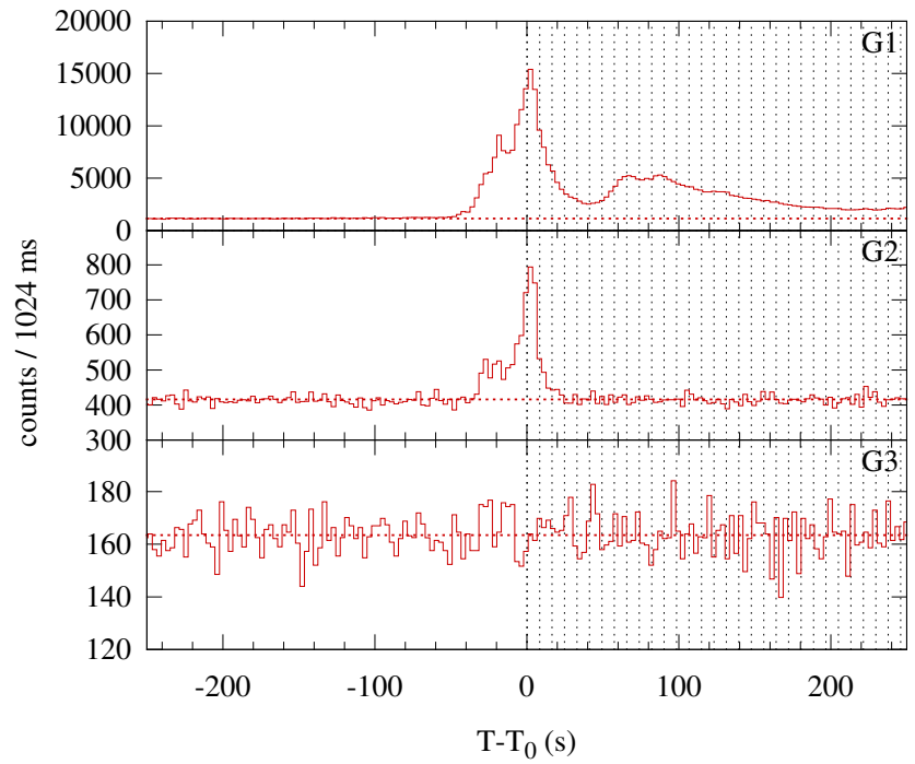
Konus-WIND S2 SOL2001-12-12T23:17 (M4.8) T 0 = 83848.429 s UT (23:17:28.429)
