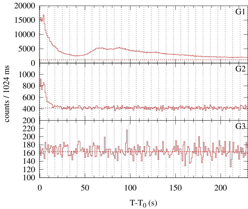
Konus-WIND S2 SOL2001-12-12T23:17 (M4.8) T 0 = 83848.429 s UT (23:17:28.429)
