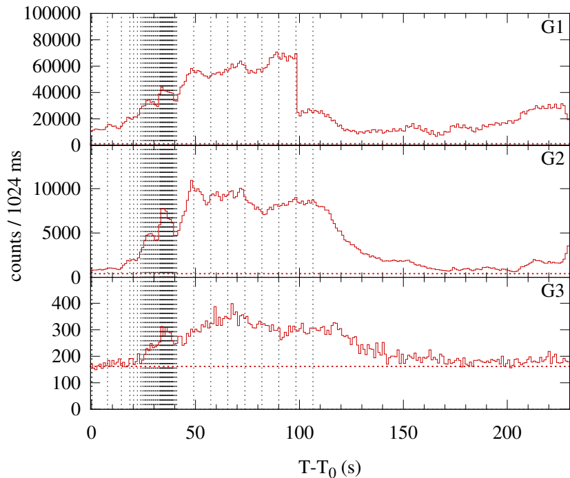
Konus-WIND S2 SOL2001-12-13T14:24 (X6.2) T_0 = 51890.76 s UT (14:24:50.76)
