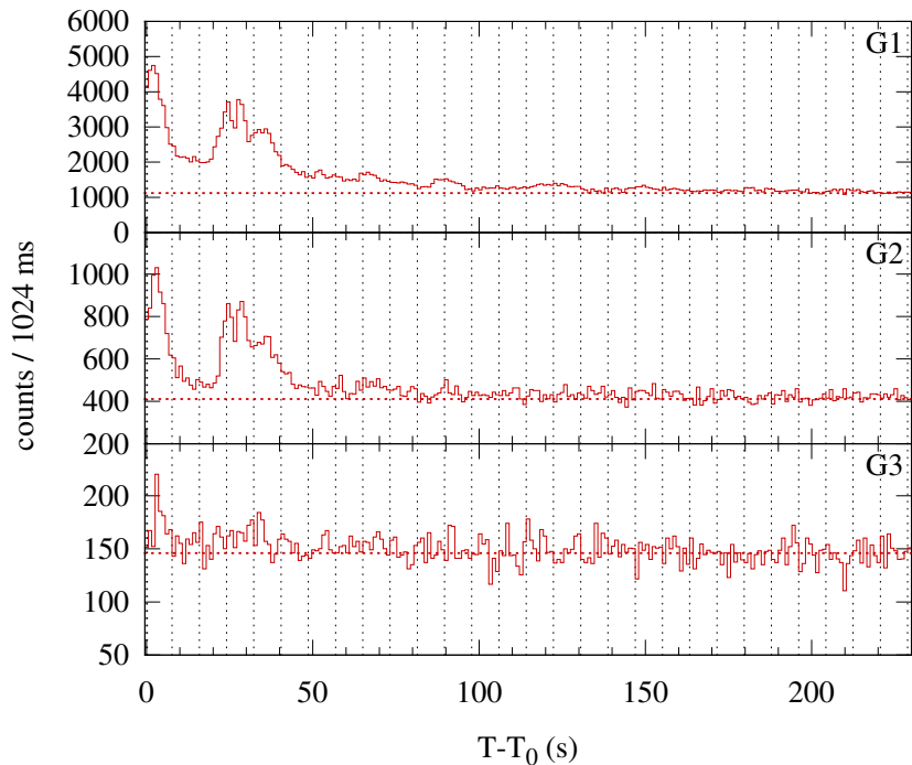
Konus-WIND S2 SOL2001-12-24T00:31 (M1.7) T 0 = 1901.895 s UT (00:31:41.895)
