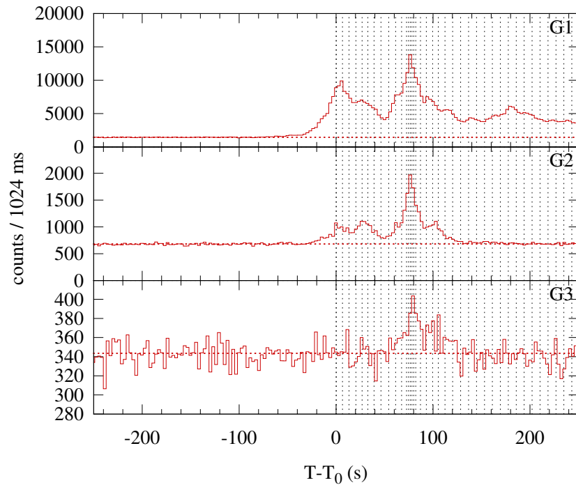
Konus-WIND S2 SOL2001-12-28T03:45 (M4.7) T 0 = 13538.6 s UT (03:45:38.6)
