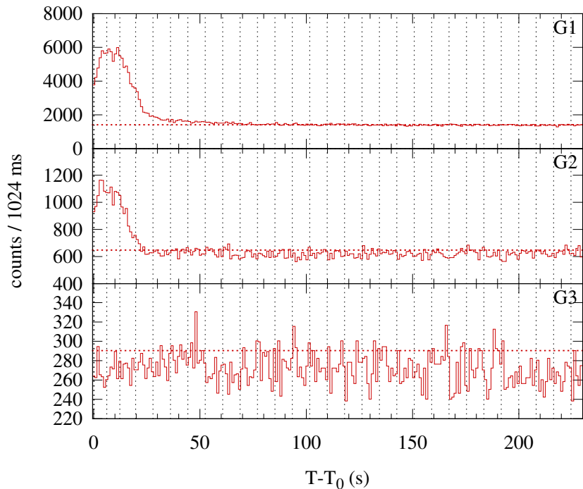
Konus-WIND S2 SOL2002-02-20T11:06 (C7.5) T_0 = 39970.74 s UT (11:06:10.74)
