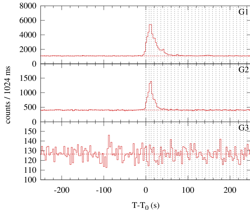
Konus-WIND S2 SOL2002-02-25T21:26 (C4.1) T 0 = 77172.884 s UT (21:26:12.884)
