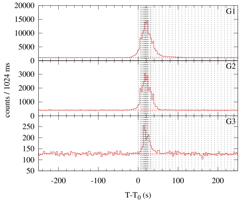
Konus-WIND S2 SOL2002-02-26T10:26 (C9.6) T 0 = 37583.466 s UT (10:26:23.466)
