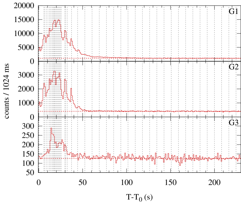
Konus-WIND S2 SOL2002-02-26T10:26 (C9.6) T 0 = 37583.466 s UT (10:26:23.466)
