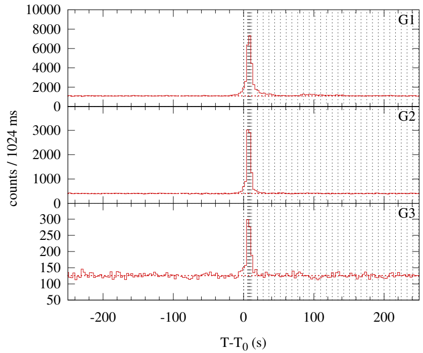
Konus-WIND S2 SOL2002-03-10T01:34 (C5.1) T 0 = 5693.874 s UT (01:34:53.874)
