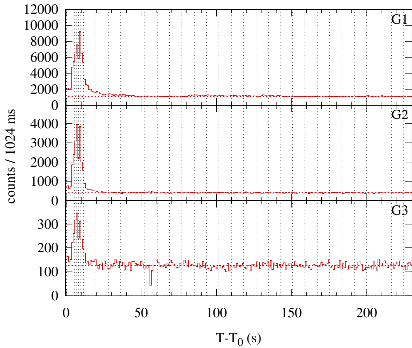
Konus-WIND S2 SOL2002-03-10T01:34 (C5.1) T 0 = 5693.874 s UT (01:34:53.874)
