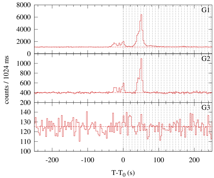
Konus-WIND S2 SOL2002-03-10T05:03 (C6.0) T_0 = 18234.269 s UT (05:03:54.269)
