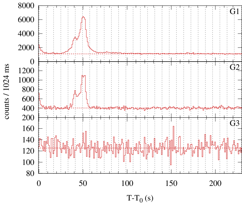
Konus-WIND S2 SOL2002-03-10T05:03 (C6.0) T_0 = 18234.269 s UT (05:03:54.269)
