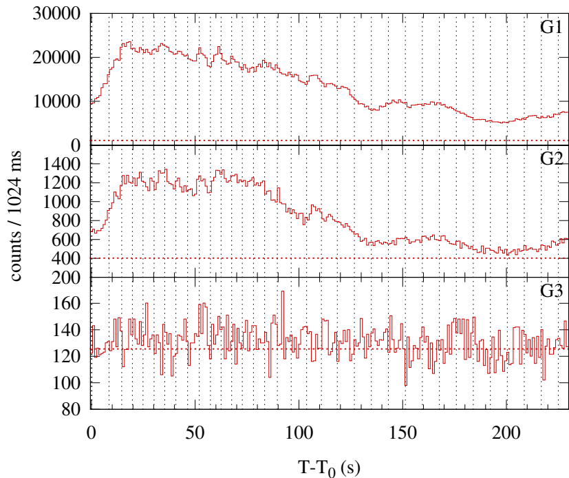
Konus-WIND S2 SOL2002-03-14T01:42 (M5.7) T_0 = 6133.93 s UT (01:42:13.93)
