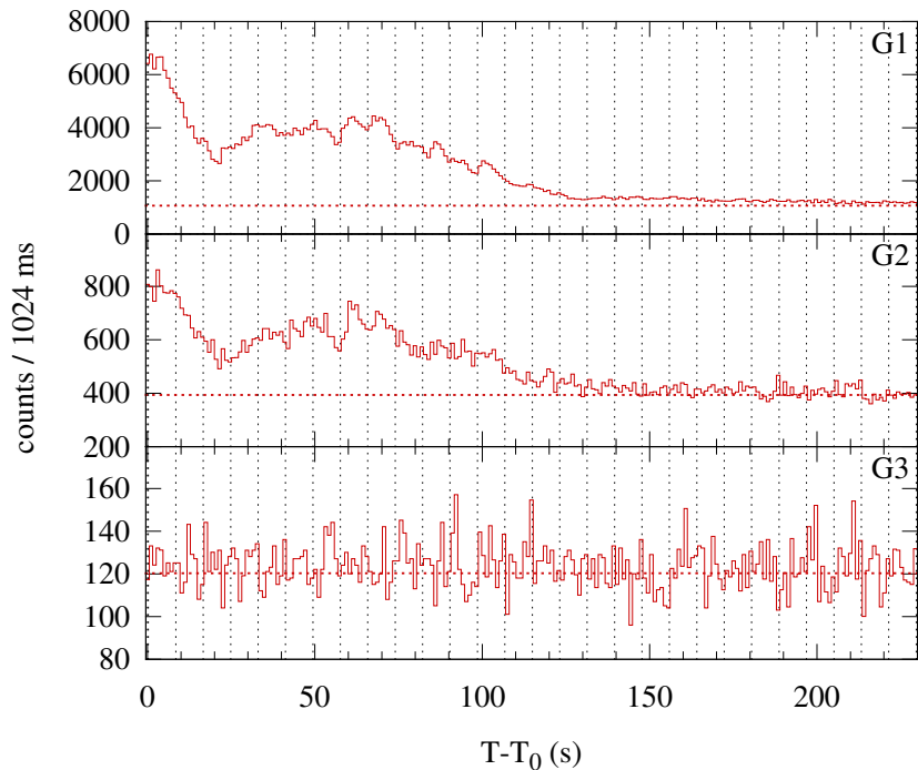
Konus-WIND S2 SOL2002-04-10T19:02 (M1.6) T_0 = 68568.908 s UT (19:02:48.908)
