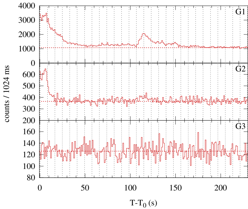
Konus-WIND S2 SOL2002-05-14T12:59 (C4.2) T 0 = 46794.410 s UT (12:59:54.410)
