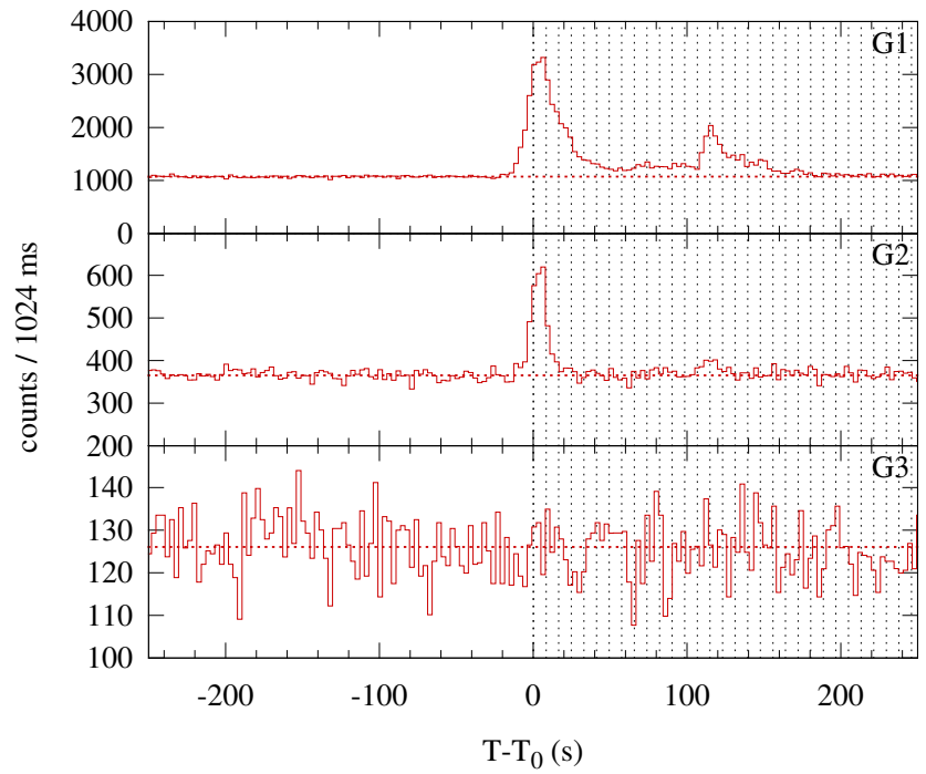
Konus-WIND S2 SOL2002-05-14T12:59 (C4.2) T 0 = 46794.410 s UT (12:59:54.410)
