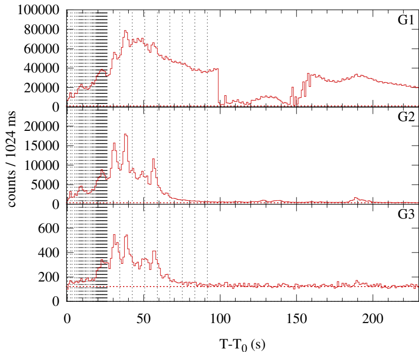
Konus-WIND S2 SOL2002-05-20T15:24 (X2.1) T_0 = 55496.403 s UT (15:24:56.403)
