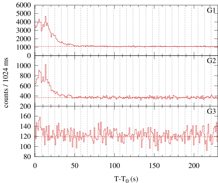
Konus-WIND S2 SOL2002-05-29T02:46 (C8.6) T 0 = 9965.45 s UT (02:46:05.45)
