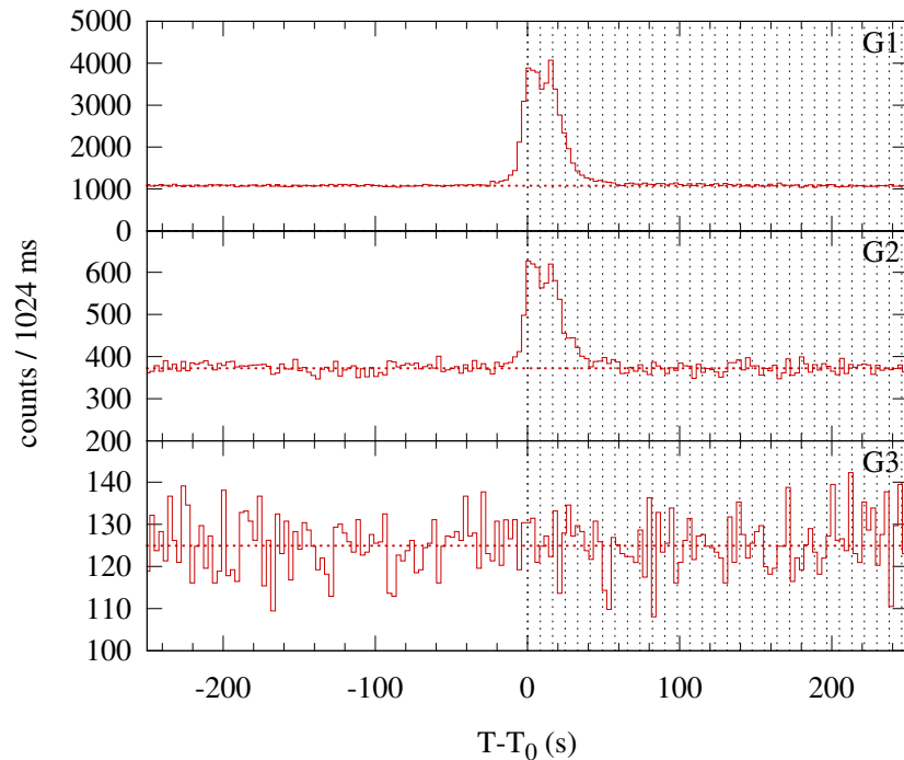
Konus-WIND S2 SOL2002-06-01T23:47 (C5.1) T_0 = 85639.279 s UT (23:47:19.279)
