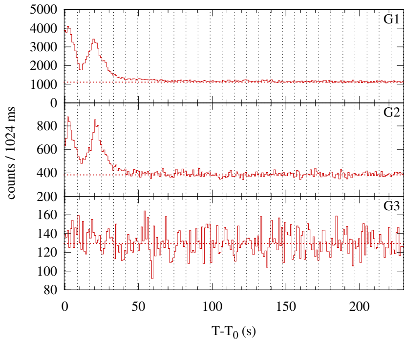
Konus-WIND S2 SOL2002-06-02T11:44 (C9.4) T 0 = 42271.685 s UT (11:44:31.685)
