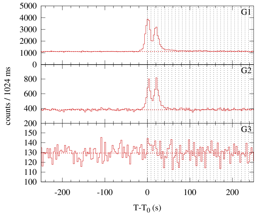
Konus-WIND S2 SOL2002-06-02T11:44 (C9.4) T 0 = 42271.685 s UT (11:44:31.685)
