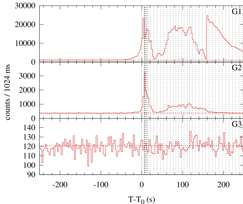
Konus-WIND S2 SOL2002-07-03T02:10 (X1.5) T_0 = 7803.233 s UT (02:10:03.233)
