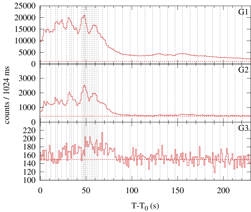
Konus-WIND S2 SOL2002-07-11T14:47 (M5.8) T_0 = 53252.737 s UT (14:47:32.737)
