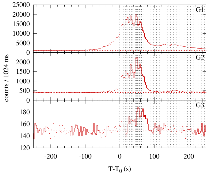
Konus-WIND S2 SOL2002-07-11T14:47 (M5.8) T_0 = 53252.737 s UT (14:47:32.737)
