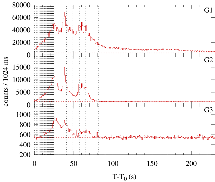
Konus-WIND S1 SOL2002-07-18T07:42 (X1.8) T_0 = 27734.161 s UT (07:42:14.161)
