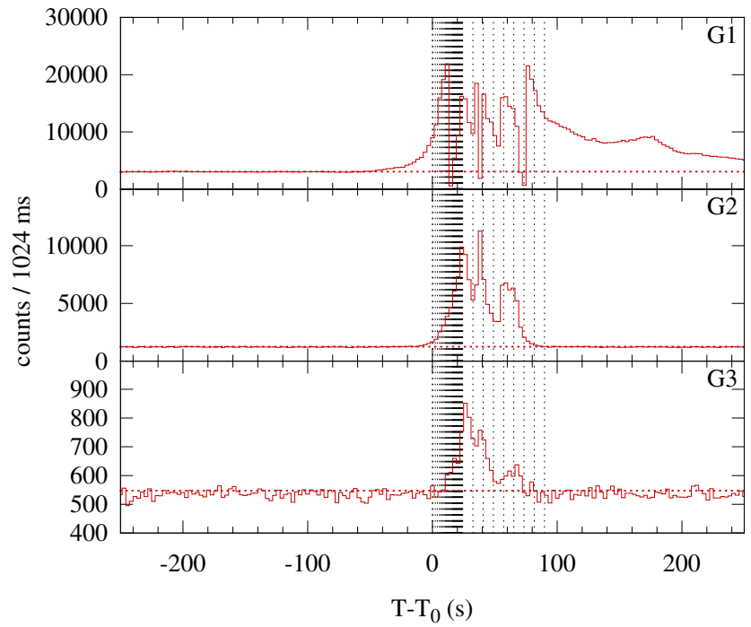
Konus-WIND S1 SOL2002-07-18T07:42 (X1.8) T_0 = 27734.161 s UT (07:42:14.161)
