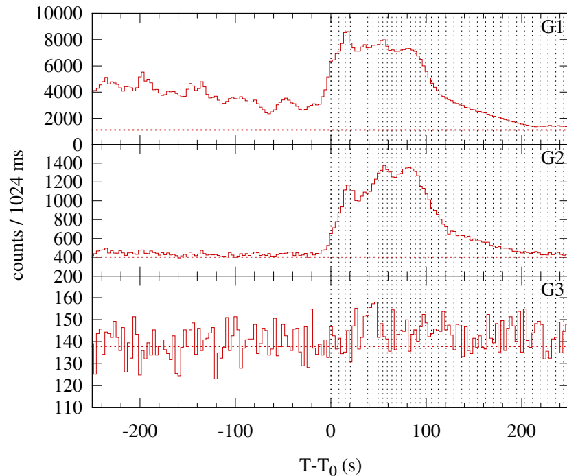
Konus-WIND S2 SOL2002-08-18T21:19 (M2.2) T 0 = 76788.274 s UT (21:19:48.274)
