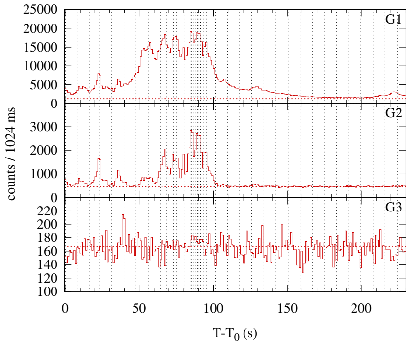
Konus-WIND S2 SOL2002-08-19T21:00 (M3.1) T_0 = 75606.240 s UT (21:00:06.240)
