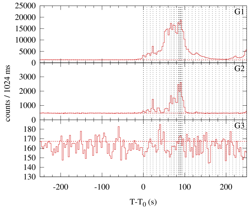
Konus-WIND S2 SOL2002-08-19T21:00 (M3.1) T_0 = 75606.240 s UT (21:00:06.240)
