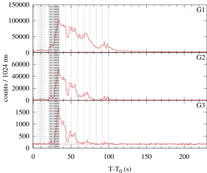
Konus-WIND S2 SOL2002-08-20T08:24 (M3.4) T_0 = 30288.249 s UT (08:24:48.249)
