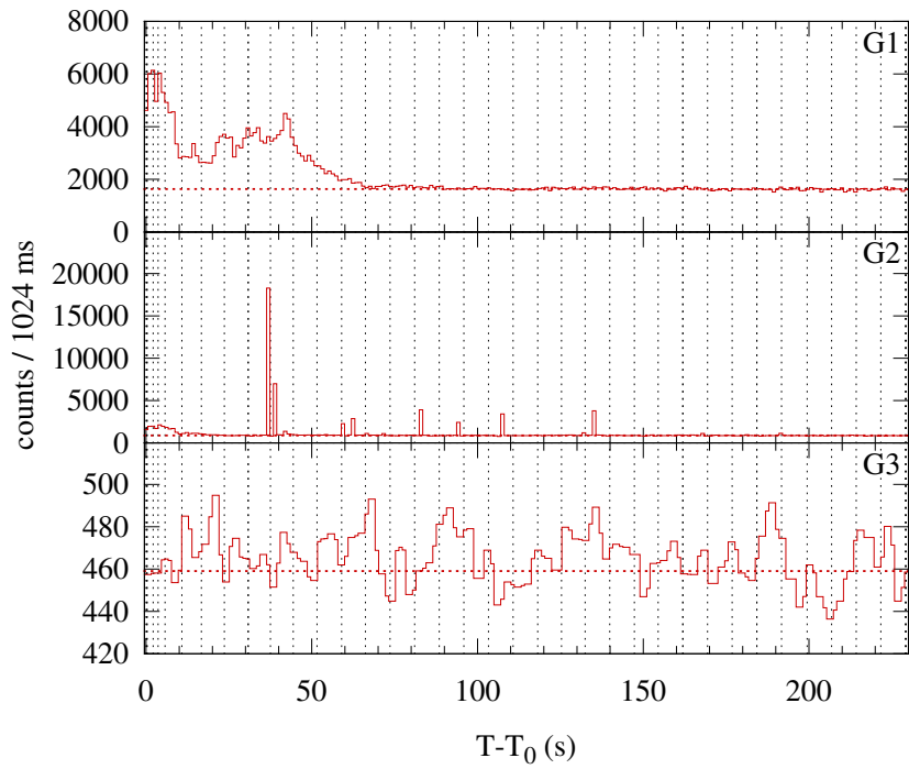
Konus-WIND S2 SOL2002-08-20T21:13 (M1.2) T 0 = 76409.396 s UT (21:13:29.396)
