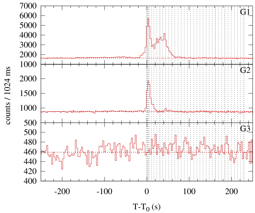
Konus-WIND S2 SOL2002-08-20T21:13 (M1.2) T 0 = 76409.396 s UT (21:13:29.396)
