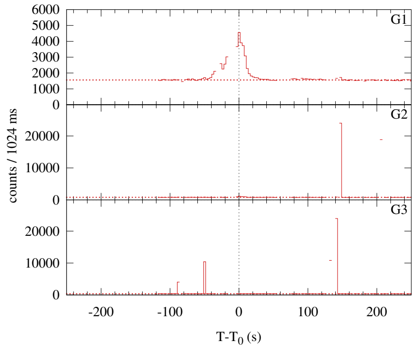
Konus-WIND S2 SOL2002-08-20T22:27 (C6.2) T_0 = 80872.468 s UT (22:27:52.468)
