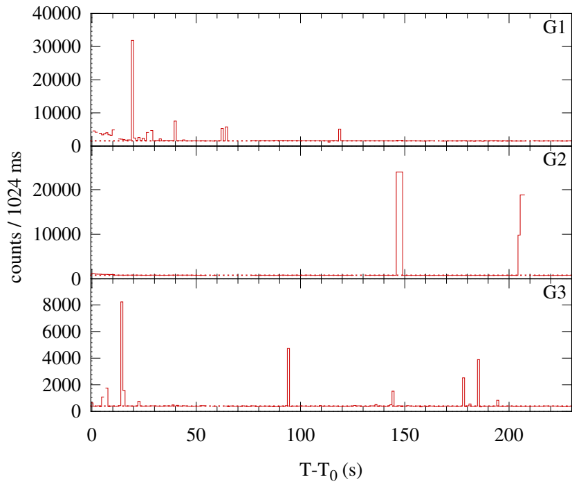
Konus-WIND S2 SOL2002-08-20T22:27 (C6.2) T_0 = 80872.468 s UT (22:27:52.468)
