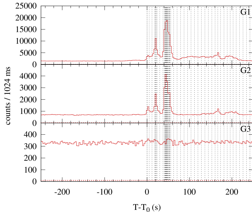
Konus-WIND S2 SOL2002-08-21T01:38 (M1.4) T_0 = 5913.242 s UT (01:38:33.242)
