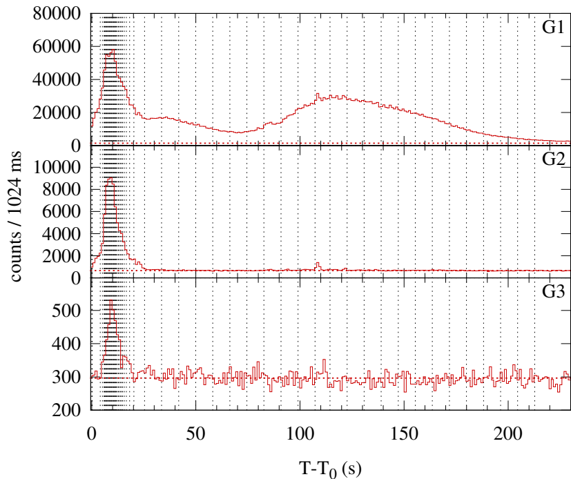
Konus-WIND S2 SOL2002-08-21T05:31 (X1.0) T_0 = 19893.781 s UT (05:31:33.781)
