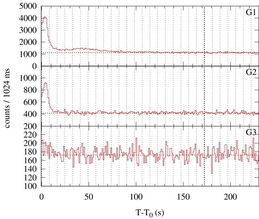
Konus-WIND S2 SOL2002-08-27T12:28 (C9.0) T_0 = 44913.932 s UT (12:28:33.932)
