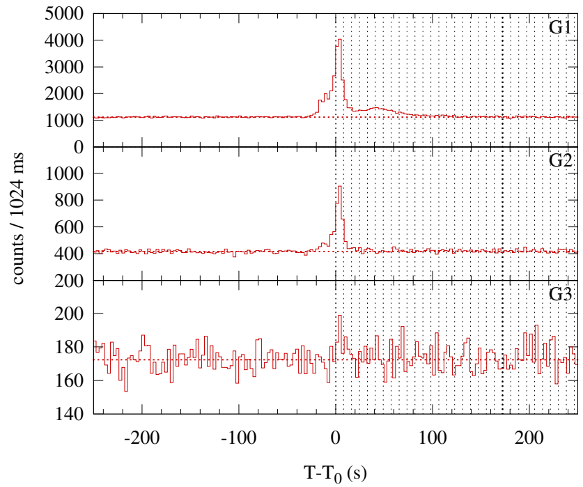
Konus-WIND S2 SOL2002-08-27T12:28 (C9.0) T_0 = 44913.932 s UT (12:28:33.932)
