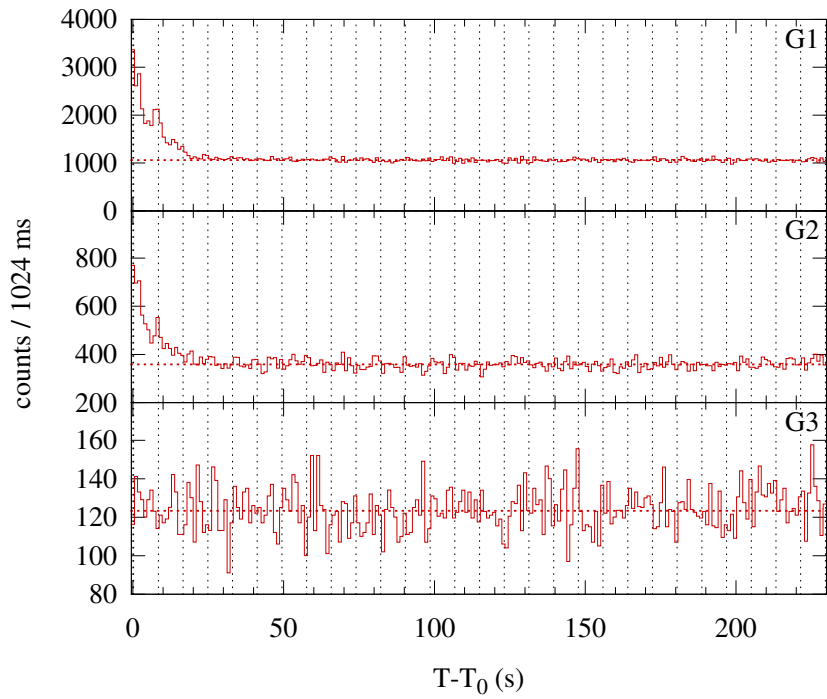
Konus-WIND S2 SOL2002-08-31T14:22 (C4.7) T 0 = 51758.460 s UT (14:22:38.460)
