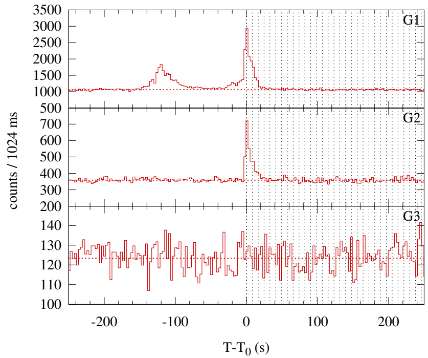
Konus-WIND S2 SOL2002-08-31T14:22 (C4.7) T 0 = 51758.460 s UT (14:22:38.460)
